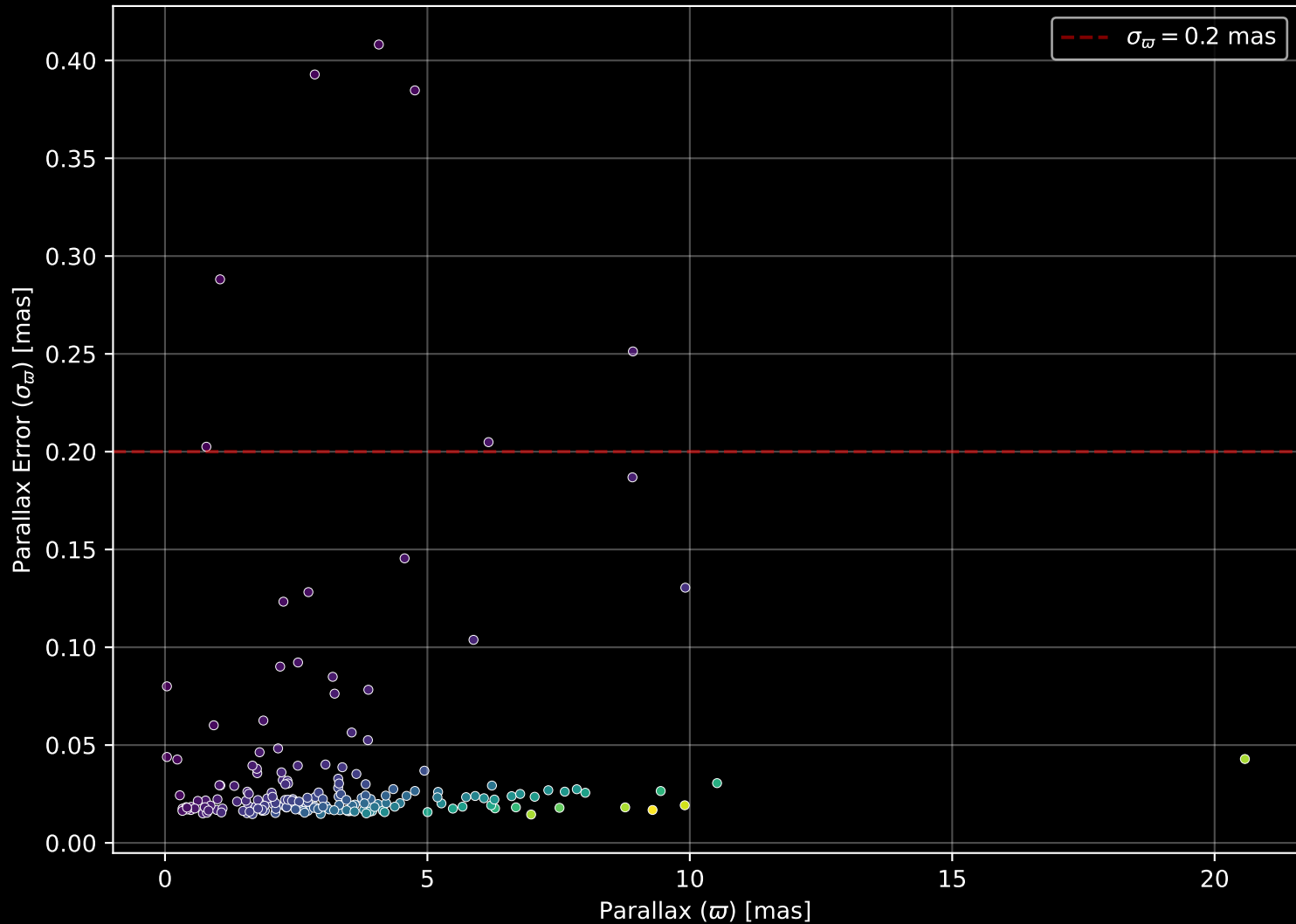
APOGEE DR17 Field: [138-62_MGA] Parallax Quality (n= 190)
