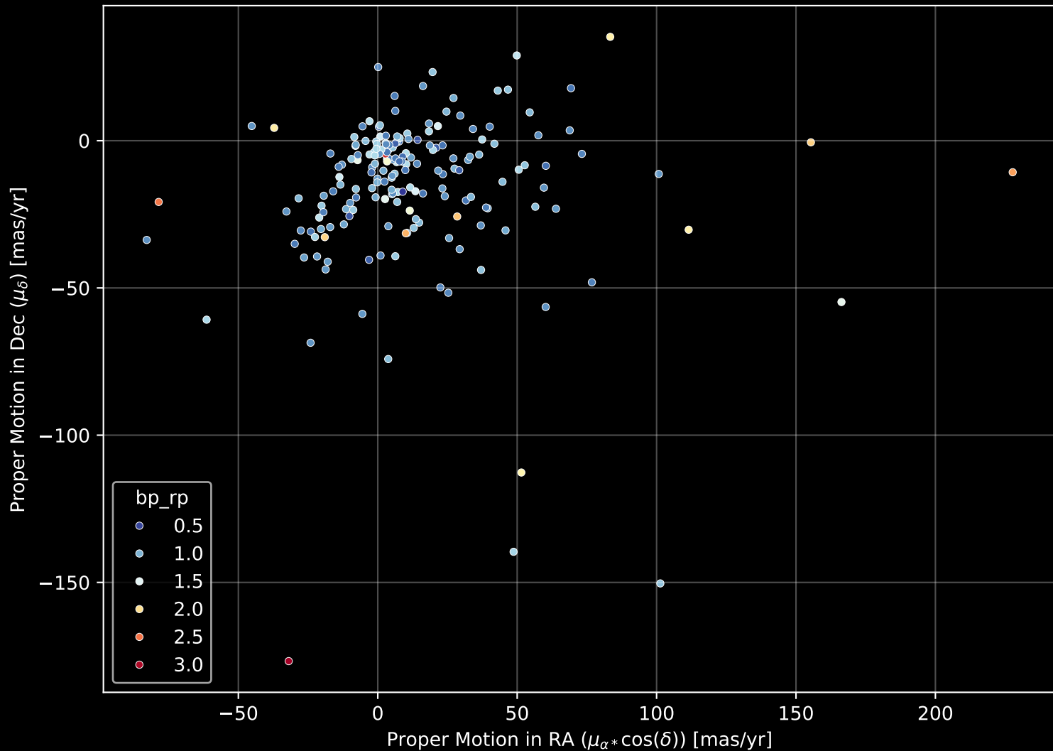
APOGEE DR17 Field: [138-62_MGA] Proper Motion Diagram (n= 190)
